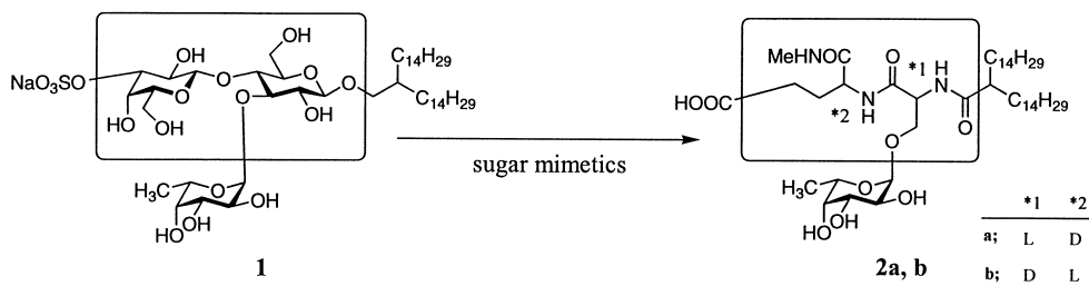
Figure 1. Successful sLe x mimetics 1 and 2a,b .
