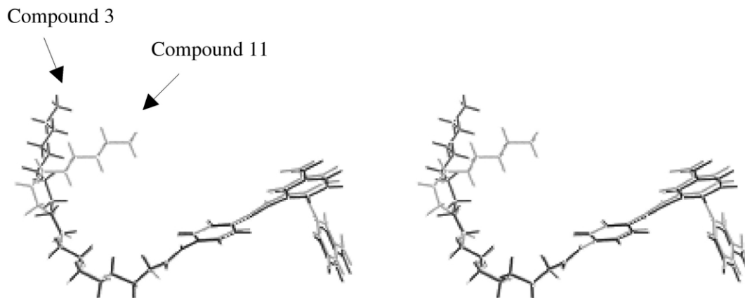
Figure 4. The stereoview of the superimpose between compounds 3 and 11 of the binding conformation toward E-selectin. The conformation of compound 3 was retrieved from the complex model with E-selectin. The conformation of compound 11 was constructed by means of changing the rotatable bonds to fit the binding conformation of compound 3 . However, the edge of the long alkyl chain of the compound 11 does not fit to that of compound 3 , because two Z-double bonds restricted the conformation. As the interaction point on E-selectin of the long alkyl chain is shallow, compound 11 cannot bind to E-selectin tightly.
