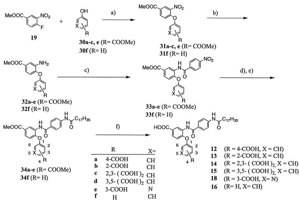
Scheme 2. Condition: (a) K_2CO_3 /DMF, 68–97%; (b) H_2 /Pd-C, 94% from 31f ; (c) 4-nitrobenzoyl chloride, Et_3N , 42–83% from 31a–c,e , 73–93% from 32d,f ; (d) H_2 /Pd-C, or 2 M SnCl_2 /DMF; (e) stearoyl chloride, Et_3N , 12–100% from 32a–e ; (f) 1 N NaOH, 23–99%.
