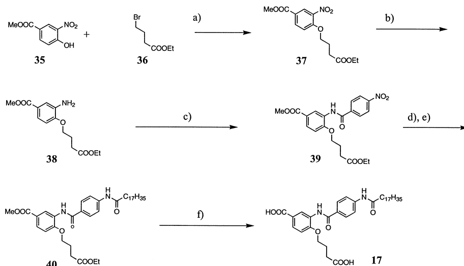
Scheme 3. Condition: (a) K_2CO_3 /DMF, 98%; (b) H_2 /Pd-C; (c) 4-nitrobenzoyl chloride, Et_3N , 91% from 37 ; (d) H_2 /Pd-C; (e) stearyl chloride, Et_3N , 87% from 39 ; (f) 1 N NaOH, 73%.
