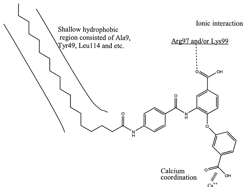
Figure 3. The scheme of the complex model of compound 3 and E-selectin based on the three points of interaction: (1) one of the carboxylic acids of isophthalic acid coordinates to calcium; (2) the carboxylic acid in the benzoic moiety forms the electric interaction with Arg97 and/or Lys99; (3) a C17 long alkyl chain interacts with the shallow hydrophobic region consisted of Leu114, Ala9, Tyr49, and so on on E-selectin.
