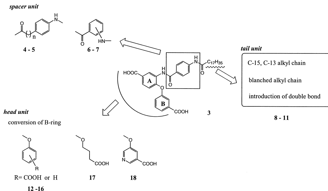
Figure 2. SAR map of non-sugar blocker ( 3 ).
